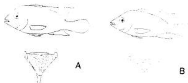
Fig. 1. A, B. Semi-schematic drawing of the differences in body shape and pharyngeal jaw morphology in C. citrinellum . Molariform morphs (A) have a shorter, blunter snout, wider head, larger eye, deeper body than papilliform morphs (B). The pharyngeal jaws are sturdier, larger, and have larger molariform teeth in molariform morphs (A) than in papilliform morphs (B).
