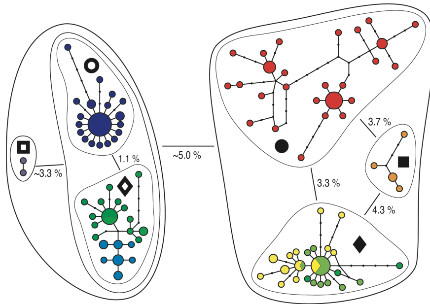
Fig. S1. Mitochondrial DNA haplotype network showing six major clades and the divergence between them, based on data described in (S1). Colors correspond to the location where each haplotype was sampled according to Fig. 1, and the area of each circle is proportional to the number of samples with that haplotype. Missing haplotypes are indicated by black dots. The symbols next to each clade indicate the symbol used on the map (Fig. 1a) that corresponds to that clade. There are two major mitochondrial clades that overlap both in central Siberia, where they delineate reproductively isolated forms (S1), and within the subspecies ludlowi in the western Himalayas, where they do not correspond to reproductively isolated forms.
