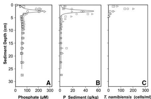
Fig. 1. Sediment profiles from the Namibian shelf (22°10'S, 14°03'E; water depth 70 m). (A) Phosphate concentrations in the pore water ( \mu\text{M} ) at different sediment depths (cm). (B) Phosphorus content of dried sediment ( \text{g kg}^{-1} ) at different sediment depths. (C) Biomass of T. namibiensis ( \text{cells ml}^{-1} ) at different sediment depths. Three parallel measurements are shown as indicated by the different symbols. The dashed lines show the steady-state concentration of pore water phosphate and the amount of phosphorus accumulation as predicted by the model calculation.
